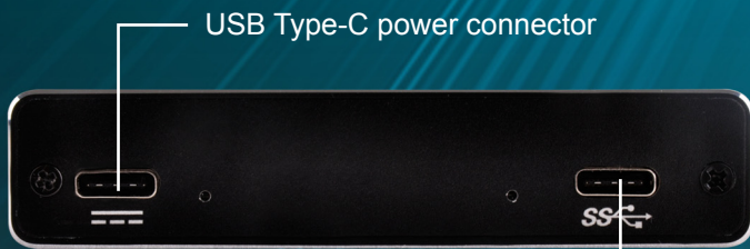
USB Type-C data connector
